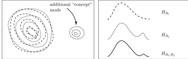
Fig. 1. Left: Illustration of two similar bag class distributions where one of the distributions, typically the positive bag distribution, has an extra mode corresponding to the positive instances. Right: Distributions of instance distances, from top to bottom: within bag instance distances in a bag from the class with no additional mode, typically the negative class; within bag instance distances in a bag from the class with an additional mode, typically the positive class. Notice the extra “bump” in the distribution; instance distances between two bags, one from each class.
